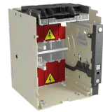
XT7-XT7M W FP 4p EF IEC/UL 1SDA104704R1
