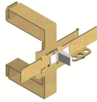
MIF T1-T2-T3 MECH, LOCK 2 C.BREAKER 1SDA051396R1
