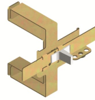
MIF T1-T2-T3 MECH, LOCK 3 C.BREAKER 1SDA052165R1
