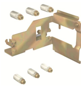
KIT MP T6 630/800 W 4p 1SDA060391R1
